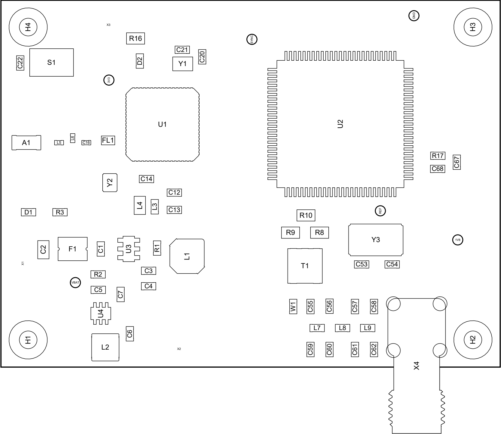
View from Top side (Scale 4:1)
