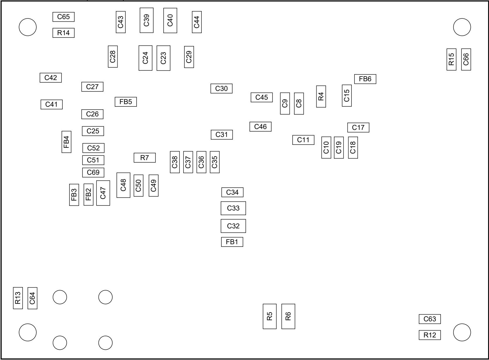
View from Bottom side (Scale 4:1)
